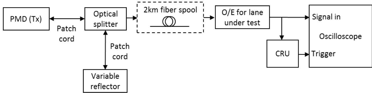
Figure 2: TDEC conformance test setup
